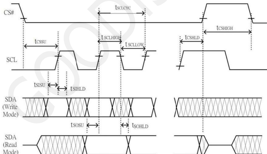
SPI interface timing
